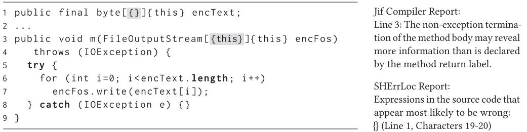
Fig. 3. Jif example. Line 3 is blamed for a mistake at line 1.
