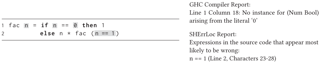
Fig. 2. Haskell example. Line 1 is blamed for a mistake at line 2.
