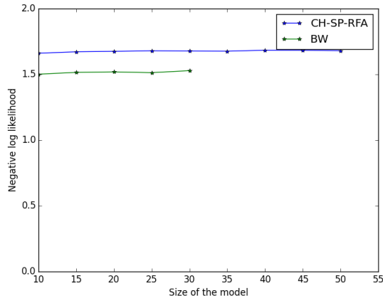
Fig. 3. Performance with the LSA representation
