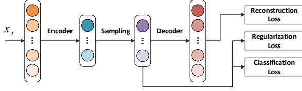
(a) VAE Training
