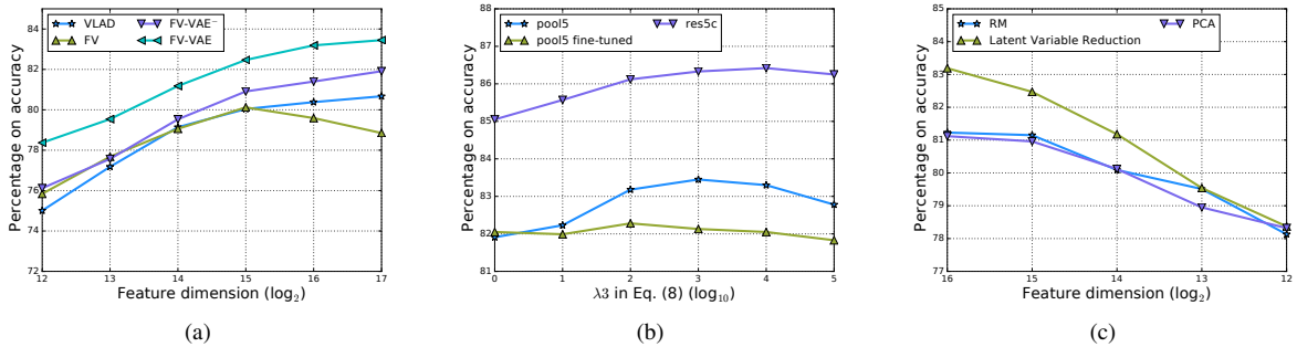
Figure 4. Experimental analysis: (a) The accuracy of visual representation with different dimensions learnt by different quantization methods. (b) The accuracy curve of FV-VAE on activations from different networks with different \lambda_3 in Eq.(8). (c) The accuracy of different feature compression methods on representation learnt by FV-VAE. Note that all the performances reported in this figure are on UCF101 split1 and similar performance trends are observed at the other two datasets.
