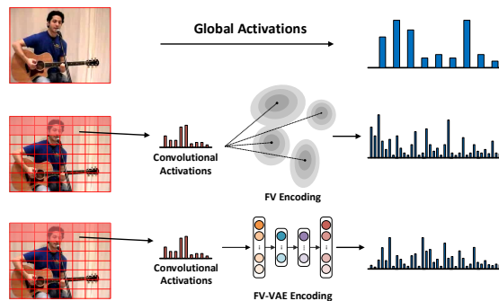
Figure 1. Visual representations derived from activations of different layers in CNNs (upper row: global activations of the fully-connected layer; middle row: convolutional activations with Fisher Vector encoding; bottom row: convolutional activations with our FV-VAE encoding).
