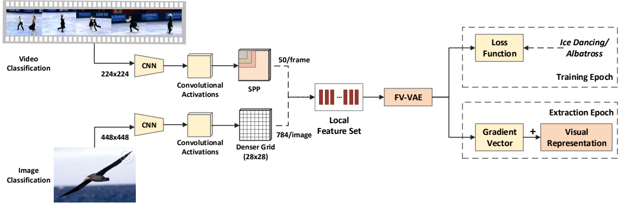
Figure 3. Visual representation learning framework for image and video recognition including our FV-VAE. Spatial Pyramid Pooling (SPP) is performed on the last pooling layer of CNN to aggregate the local descriptors of video frame, which applies four different max pooling operations and obtain (6 \times 6) , (3 \times 3) , (2 \times 2) and (1 \times 1) outputs for each convolutional filter, resulting a total of 50 descriptors. For image, an input with a higher resolution of (448 \times 448) is fed into the CNN and the activations of the last convolutional layer conv 5.4 +relu in VGG_19 are extracted, leading to dense local descriptors of 28 \times 28 . In training stage, FV-VAE architecture is learnt by minimizing the overall loss. In extraction epoch, the learnt FV-VAE is to encode the set of local descriptors into a vectorial FV representation.
