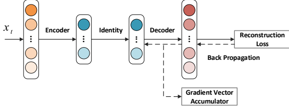
(b) FV Extraction
