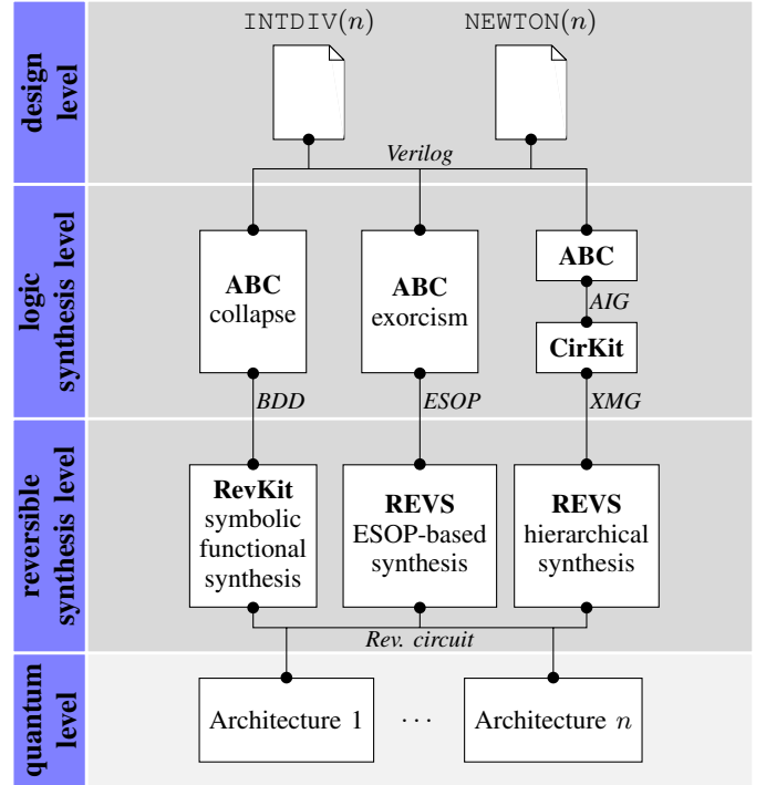
Fig. 1. Design flows; lines represent interfaces between files and tools and are annotated using the function representation at the interface
