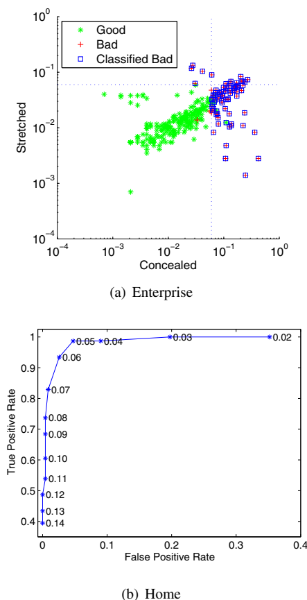
Fig. 15. Classifier Results Using RTAudio 16k.
