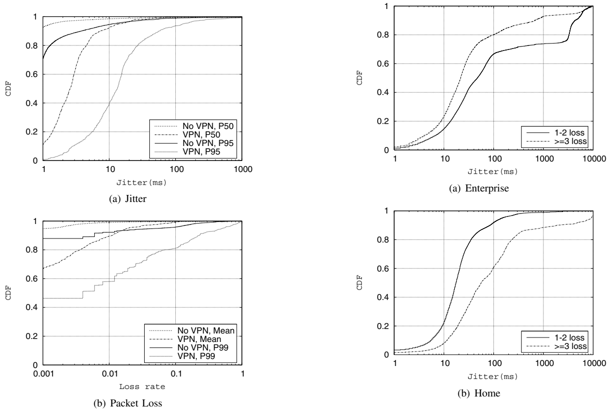
Fig. 14. The correlation between loss and jitter. End-to-end delay increases significantly before loss events in both enterprise and home networks.
