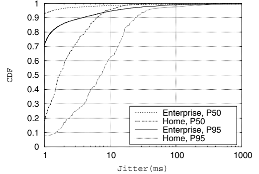
Fig. 7. Jitter Distribution (US-US, wired traces).
