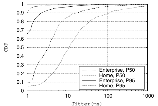
Fig. 8. Jitter Distribution (inter-continental, wired traces).
