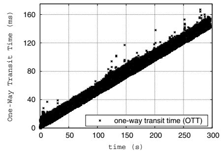
Fig. 3. Clock Skew in the Wild
