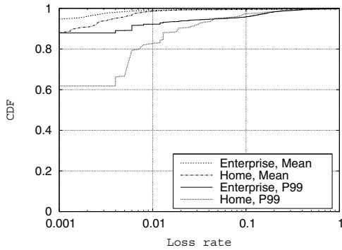
Fig. 9. Loss Rate Distribution (US-US, wired traces).
