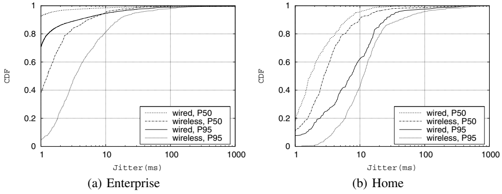
Fig. 11. Impact of WiFi Connections on Jitter.
