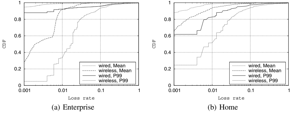
Fig. 12. Impact of WiFi Connections on Packet Loss.
