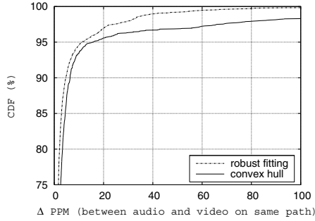
Fig. 4. Comparison of Skew Estimation Algorithms
