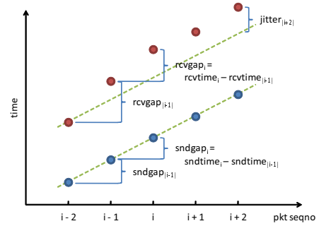
Fig. 5. Jitter calculation
