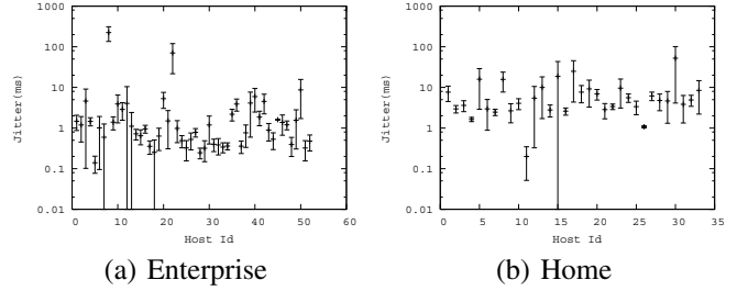
Fig. 1. Jitter distribution across hosts.
