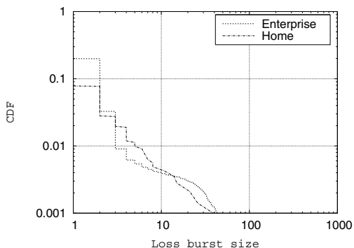
Fig. 10. Loss Burst Size Distribution (US-US, wired traces).
