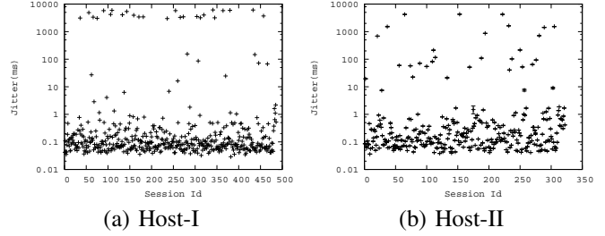
Fig. 2. Jitter distribution across sessions.
