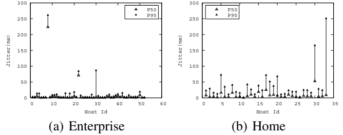
Fig. 6. The 50 th and 95 th percentile of jitter distribution across hosts. Jitter variation is much higher in residential networks than in enterprise networks. Figure 6(b) shows that 95 th percentile jitter values is significantly worse than the median jitter values in home networks.
