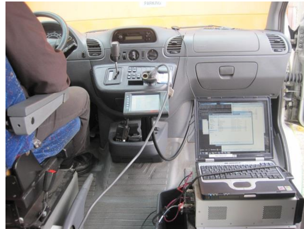
Shuttle Setup
