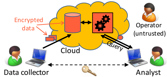
Figure 1: Motivating scenario.
