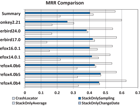
Figure 7. The comparisons between CrashLocator and three stack-only methods (MRR).
