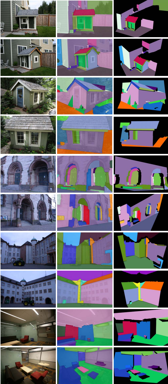
Figure 7. Results from the PLAYHOUSE, SHED, ARCHES, CASTLE and ROOM datasets. For each one of these datasets, we show two sets of the original image, the recovered depth map (colors indicate different planes) and the corresponding mesh rendered from a new viewpoint. Note the accurate polygonal boundaries especially the straight creases between adjoining polygons that meet.
