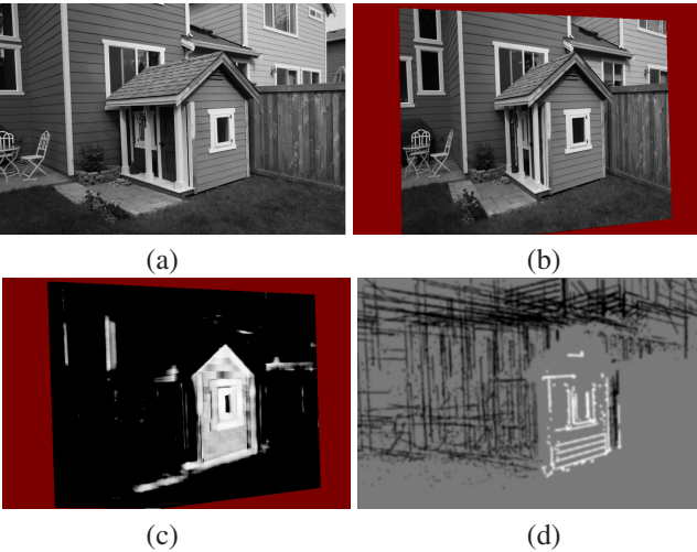
Figure 5. [Top] A 3D point X and line segment L are inliers to plane m_i while their ray-visibility imposes free-space violation penalties for plane m_k . (a,b) Image pair registered via plane induced homography. (c) Photo-consistency measure: White (black) denotes high (low) scores while unknown pixels are red. (d) Free space violation penalties (black) and inlier constraints (white).
