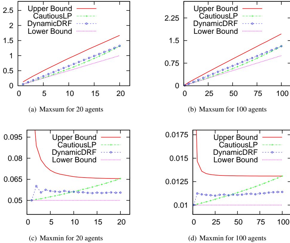
Figure 3: The maxsum and maxmin objectives as a function of the time step k , for n = 20 and n = 100 .
