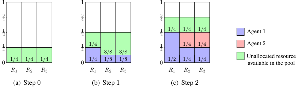
Figure 1: Allocations returned by DYNAMIC DICTATORSHIP on the instance described in Example 2.
