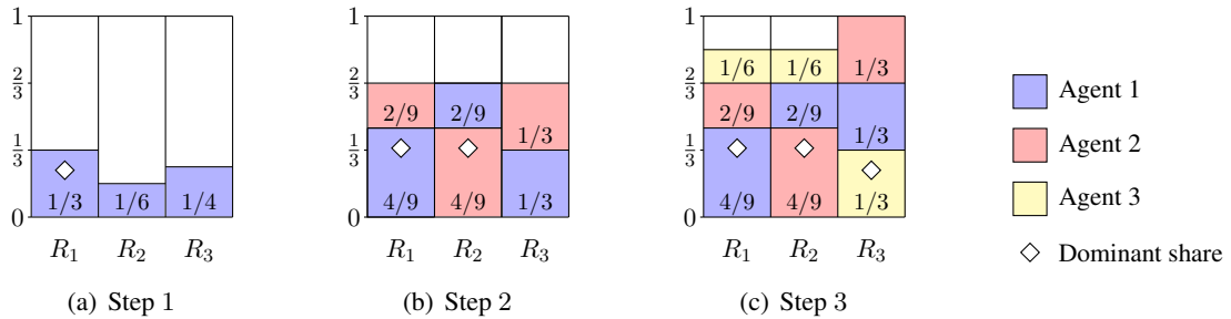
Figure 2: Allocations returned by DYNAMIC DRF at various steps for 3 agents with demands \mathbf{d}_1 = \langle 1, 1/2, 3/4 \rangle , \mathbf{d}_2 = \langle 1/2, 1, 3/4 \rangle , and \mathbf{d}_3 = \langle 1/2, 1/2, 1 \rangle , and three resources R_1, R_2 , and R_3 . Agent 1 receives a 1/3 share of its dominant resource at step 1. At step 2, water-filling drives the dominant shares of agents 1 and 2 up to 4/9 . At step 3, however, agent 3 can only receive a 1/3 dominant share and the allocations of agents 1 and 2 remain unchanged.
