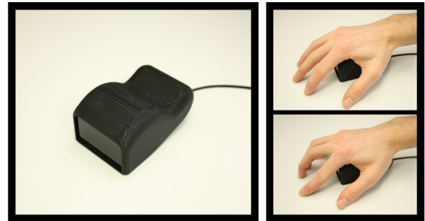
Figure 10. Side Mouse rests under the palm of hand, allowing fingers to touch the table surface directly in front of the device. These are sensed using an internal camera and IR laser.
