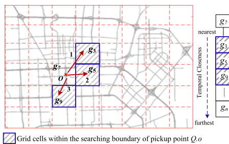
Fig. 7. The single-side taxi searching algorithm.
