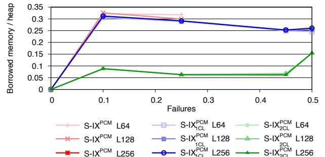
(b) Two-page clustering greatly reduces dependency on borrowed pages.
