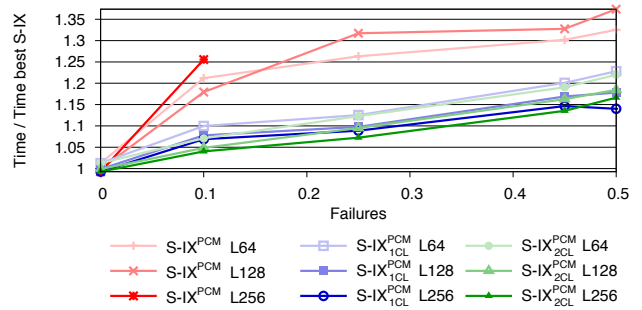
(a) Hardware failure clustering greatly improves performance.
