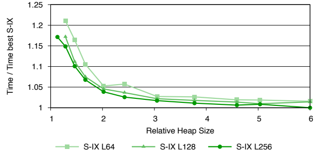
(a) The effect of line size on baseline S-IX.
