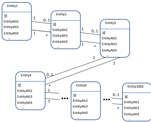
Figure 8: Chain model
