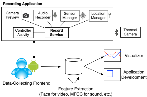
Figure 1: Overview of the workflow
