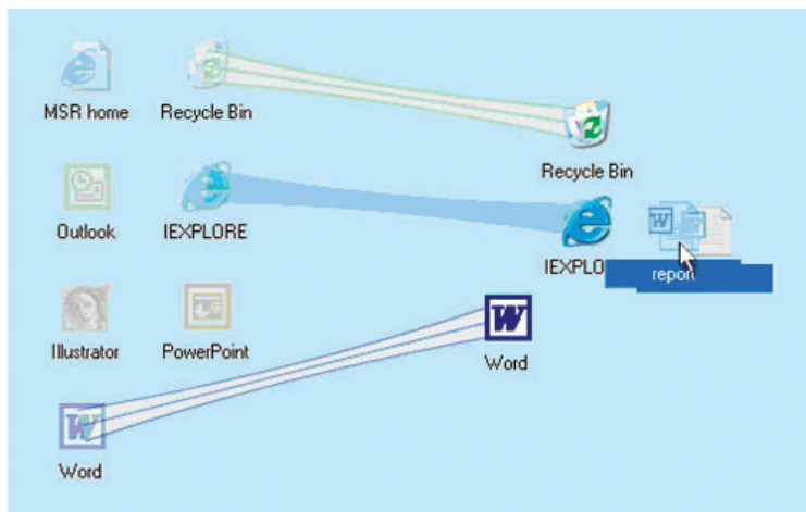
2 Drag-and-Pop interaction. To preserve users' spatial memory, the technique stretches the potential targets toward the object being dragged.
