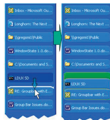
7 GroupBar technology. Dragging a window tile onto another tile combines both into a group.
