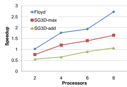
Figure 9. Floyd and SG3D.
