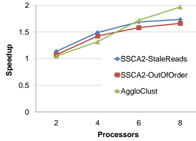
Figure 8. SSCA2 and AggloClust.
