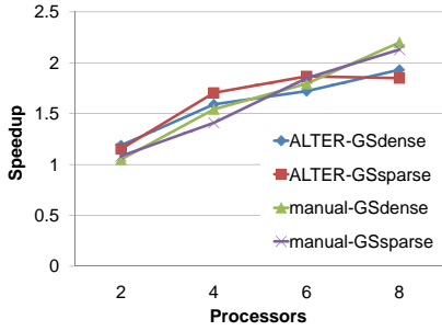
Figure 10. Dense and sparse linear algebra.
