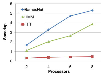
Figure 11. BarnesHut, FFT, and HMM.
