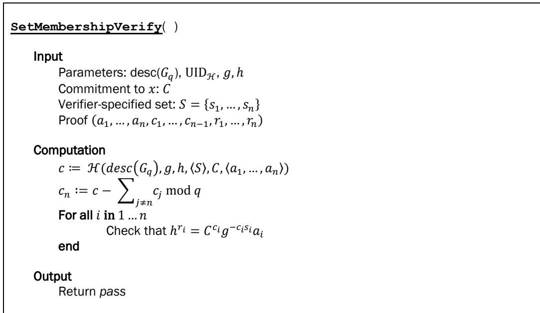
Figure 2: SetMembership Verify
