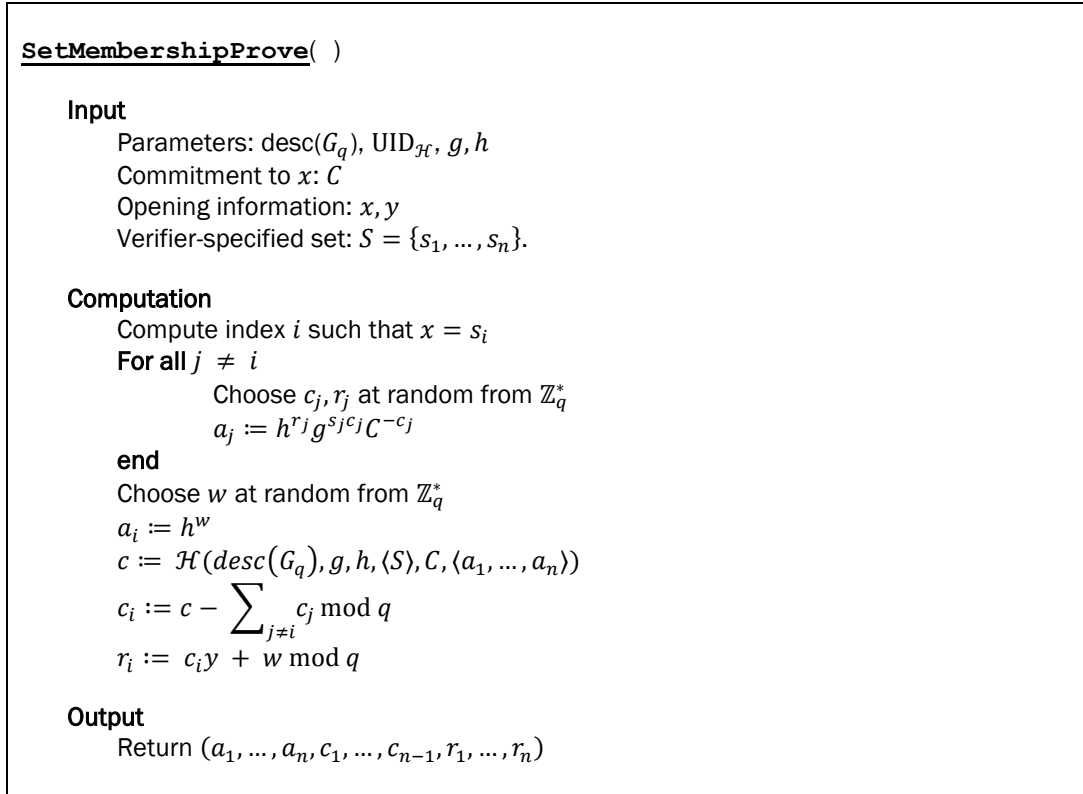
Figure 1: SetMembershipProve
