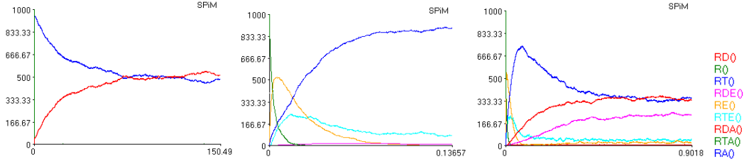
Fig. 5. SPiM plots of simulations for Figure 7 and 15. The x -axis is the time in minutes and y -axis is the number of processes. The legend on the right is for all the three plots, where red, green, blue, pink, yellow, and light blue colours are used for RD, R, RT, RDE, RE, and RTE molecules, respectively.
