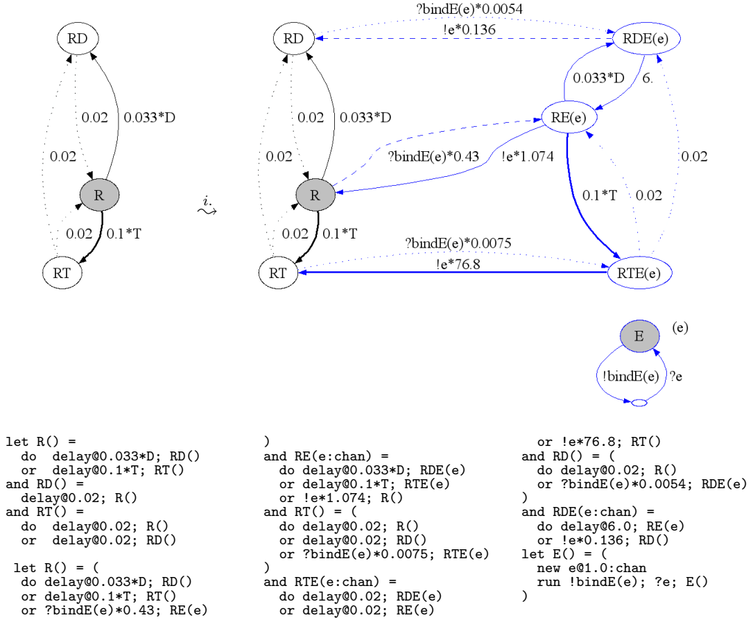
Fig. 7. Compositional construction of the process model for the Rho GTP-binding proteins with GEF and without GAP with respect to \overset{i}{\sim} in Figure 4.
