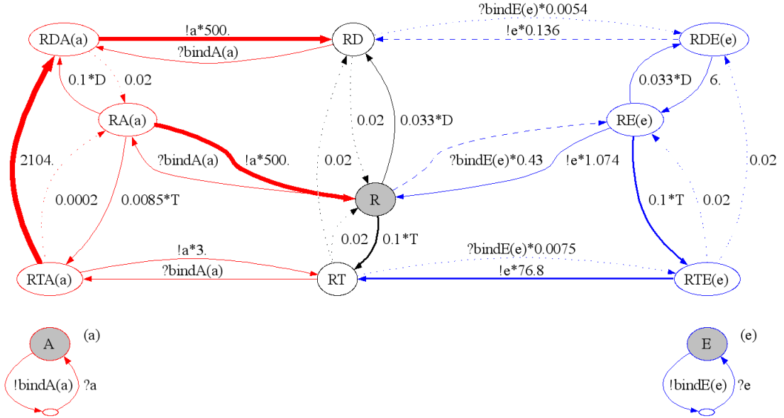
Fig. 9. Compositional construction of the process model for the Rho GTP-binding proteins with GEF and GAP with respect to \rightsquigarrow in Figure 4.
