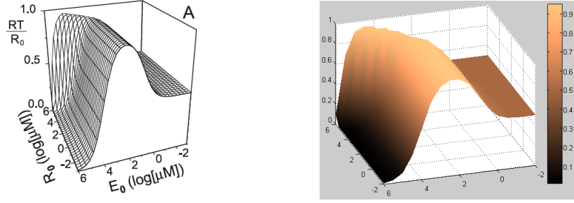
Fig. 8. Graphs displaying the RT/R_0 ratio as the output of the ODE [13] and process simulations, respectively, for the models for Rho GTP-binding proteins with GEF and without GAP.
