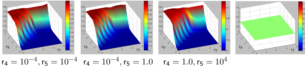
Fig. 17. The result of the simulations with respect to RT/R_0 ratio at the z -axis, where R_0 and E_0 are set to 1000. A_0 is 10 and G_0 is 600. The x and y -axis are the parameters for the reactions r_6 and r_7 varying between 10^{-4} and 10^4 . For the case where r_4 = 10^{-4} and r_5 = 10^4 , we observe a plot similar to those on the left above. We observe a plateau at 0.1, as in the right-most plot, for the cases where r_4 = 1.0 , r_5 = 1.0 ; r_4 = 10^4 , r_5 = 10^4 ; r_4 = 10^4 , r_5 = 1.0 ; r_4 = 10^4 , r_5 = 10^{-4} and r_4 = 1.0 , r_5 = 10^{-4} .
