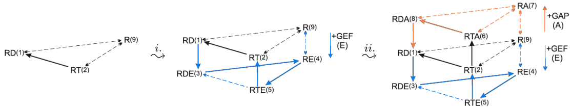
Fig. 4. A graphical representation of modular construction of the interactions of Rho GTP-binding proteins with respect to the ODE model in [13]. A basic model excluding the regulators GEF (E) and GAP (A) is extended first with GEF ( i. ) and then with GAP ( ii. ).
