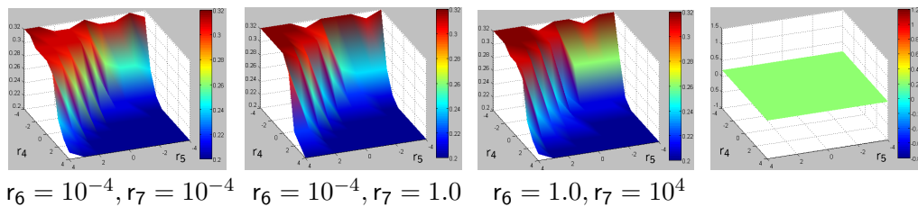
Fig. 18. The result of the simulations with respect to RT/R_0 ratio at the z -axis, where R_0 and E_0 are set to 1000. A_0 is 10 and G_0 is 300. The x and y -axis are the parameters for the reactions r_4 and r_5 varying between 10^{-4} and 10^4 . For the case where r_6 = 10^{-4} and r_7 = 10^4 , we observe a plot similar to those on the left above. We observe a plateau at 0.2, as in the right-most plot, for the cases where r_6 = 1.0 , r_7 = 10^{-4} ; r_6 = 1.0 , r_7 = 1.0 ; r_6 = 10^4 , r_7 = 10^{-4} ; r_6 = 10^4 , r_7 = 1.0 and r_6 = 10^4 , r_7 = 10^4 .
