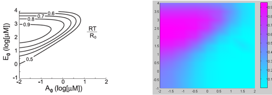
Fig. 10. Graphs displaying the RT/R_0 ratio as the output of the ODE [13] and process simulations, respectively, for the models for Rho GTP-binding proteins with GEF and GAP.
