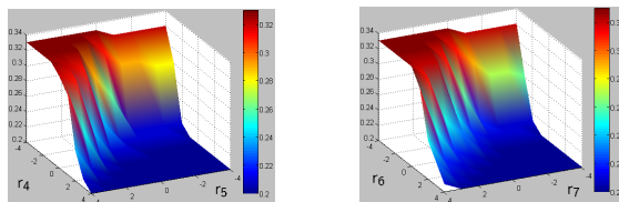
Fig. 19. The result of the simulations with respect to RT/ R_0 ratio at the z -axis, where R_0 and E_0 are set to 1000. A_0 is 10 and G_0 is 300. In the simulations on the left-hand-side, the reactions r_6 and r_7 are removed from the system, and on the right-hand-side, the reactions r_4 and r_5 are removed. The x and y -axis are the parameters for the reactions r_4 and r_5 on the left, and for the reactions r_6 and r_7 on the right, varying between 10^{-4} and 10^4 .
