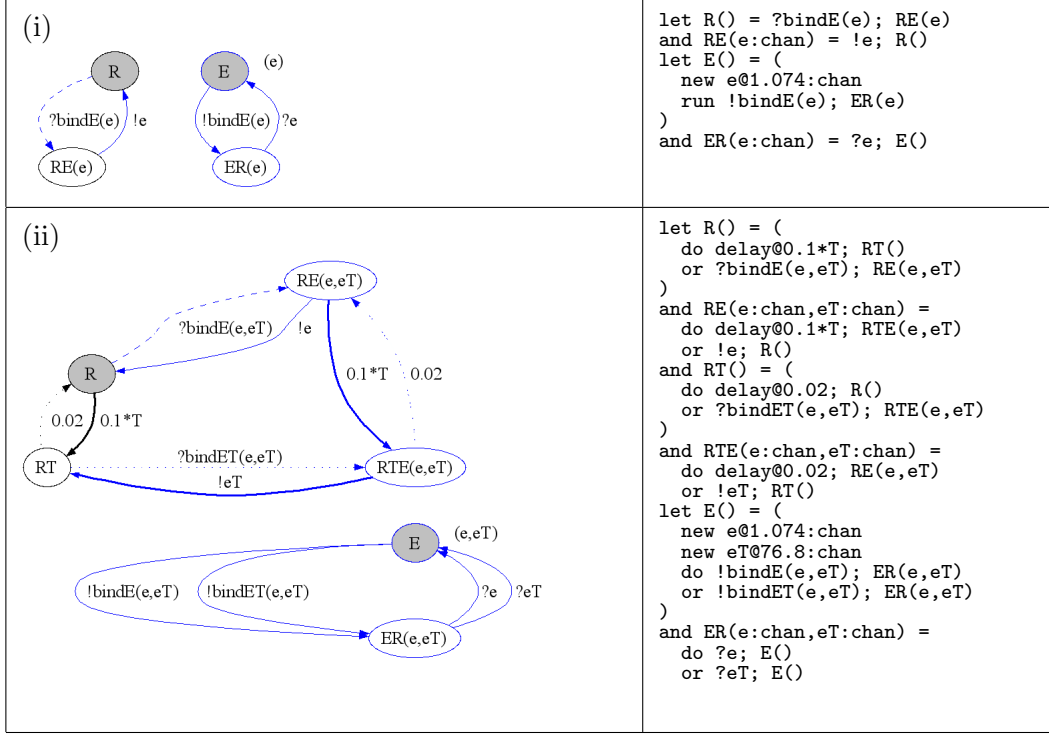
Fig. 6. An example for the progressive refinement of a stochastic \pi -calculus model of Rho GTP binding with GEF. For each of the models, the graphical representation on the left is equivalent to the textual representation on the right.
