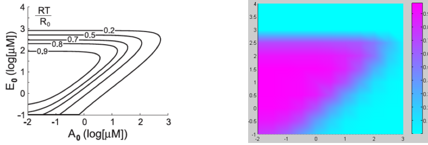
Fig. 11. Graphs displaying the RT/R_0 ratio as the output of the ODE [13] and process simulations, respectively, for the models for Rho GTP-binding proteins with GEF, GAP and effectors.
