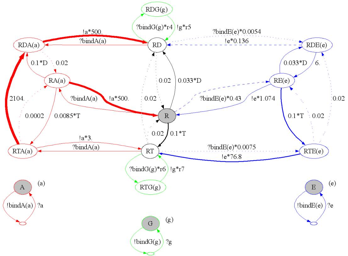
Fig. 15. The graphical representation of the model with GDIs, extending the model depicted in Figure 9.
