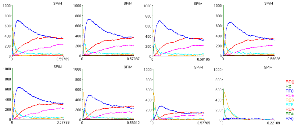
Fig. 16. SPiM plots of simulations with the model which extends GTP-binding protein cycle with GDI and effectors. The x -axis is the time in minutes and y -axis is the number of processes. The legend on the right is for all the the plots. In all the simulations, R_0 and E_0 are 1000; A_0 is 10. From left to right, the G_0 value is 0, 10, 30, 60, 100, 300, 600 and 1000.
