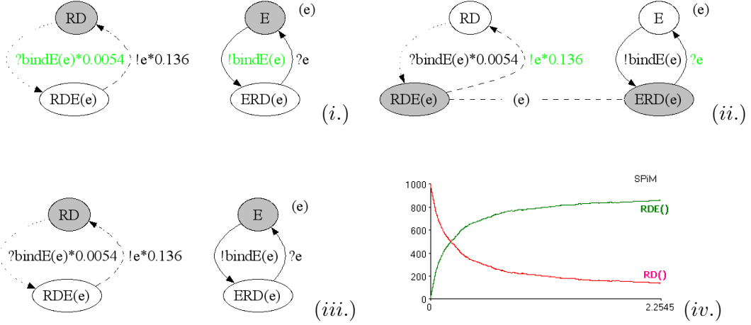
Fig. 3. Graphical representation of the evolution of the RD and E interaction model. Processes RD and E coexist and they can interact on channel bindE (i.). When they interact, E sends the private channel e , and RD receives it. This way, they evolve to processes ERD( e ) and RDE( e ), respectively, which share the private channel e , representing a bond between two bio-chemical species (ii.). By interacting on channel e , they evolve back to the processes E and RD, respectively (iii.). The SPiM plots of a simulation of the process are shown in (iv.) The x -axis is the time in minutes and y -axis is the number of processes. The simulation is started with 1000 RD and 1000 E.
