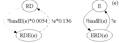
Fig. 3. Graphical representation of the evolution of the RD and E interaction model. Processes RD and E coexist and they can interact on channel bindE (i.). When they interact, E sends the private channel e , and RD receives it. This way, they evolve to processes ERD( e ) and RDE( e ), respectively, which share the private channel e , representing a bond between two bio-chemical species (ii.). By interacting on channel e , they evolve back to the processes E and RD, respectively (iii.). The SPiM plots of a simulation of the process are shown in (iv.) The x -axis is the time in minutes and y -axis is the number of processes. The simulation is started with 1000 RD and 1000 E.
