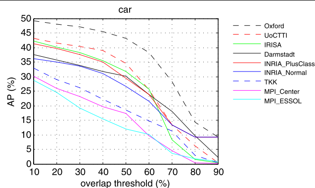
Fig. 19 Effect of the bounding box overlap threshold on the AP measure. For the class “car”, on which the submitted methods gave the best results, AP is plotted as a function of the overlap threshold. The threshold adopted for the challenge is 50%
