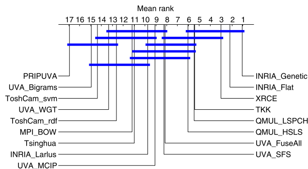
Fig. 8 Analysis of statistically significant differences in the classification results. The mean rank over all classes is plotted on the x -axis for each method. Methods which are not significantly different ( p = 0.05 ), in terms of mean rank, are connected
