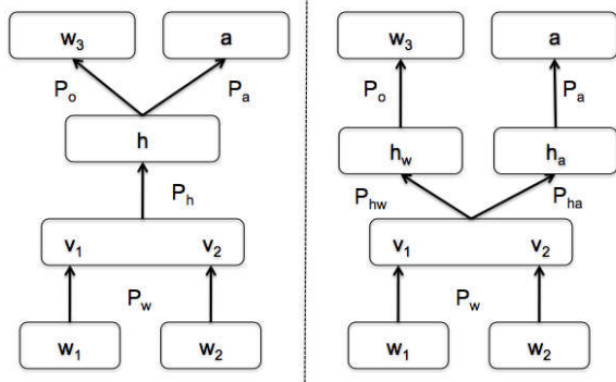
Figure 2: Models for joint training. The left pane shows joint training with separate output parameters for word and addressee labels, while the right pane shows joint structure with separate word-vector to hidden weights.
