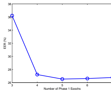
Figure 4: Effect of Phase 1 Training on Addressee Detection Task. The x-axis denotes the number of Phase 1 training epochs on Fisher, ICSI, and CB corpora, and y-axis is EER.
