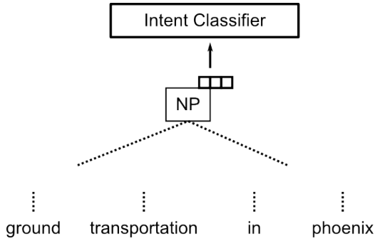
Fig. 2. The intent classifier
