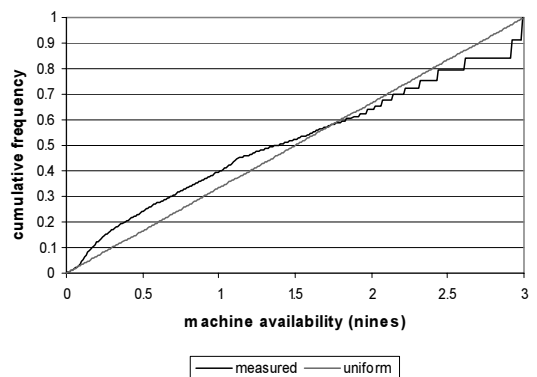
Figure 1. Machine availability distribution
