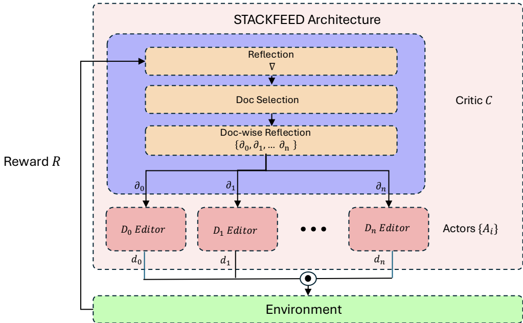
Figure 2: STACKFEED Multi-actor, centralized critic architecture: On receiving a reward from the environment, the critic generates a reflection over the failures to calculate the textual gradient \nabla . The critic uses this reflection to select the documents responsible for the error and proceeds to assign credit to the actors in the form of document-wise reflections. The actors then proceed to iteratively edit the documents. All the document-wise edits are then pooled to define the KB edit.
