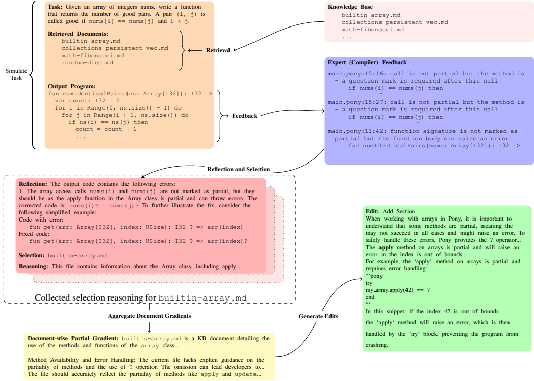
Figure 1: Example of the STACKFEED in the ARKS Pony scenario
