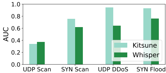
Figure 3: AUC scores with flow traces
