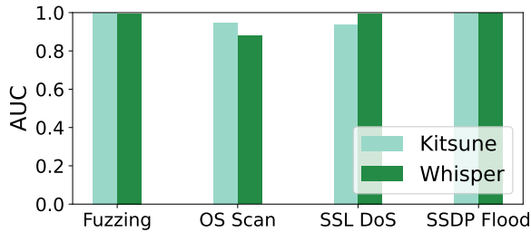
Figure 2: AUC scores with packet traces
