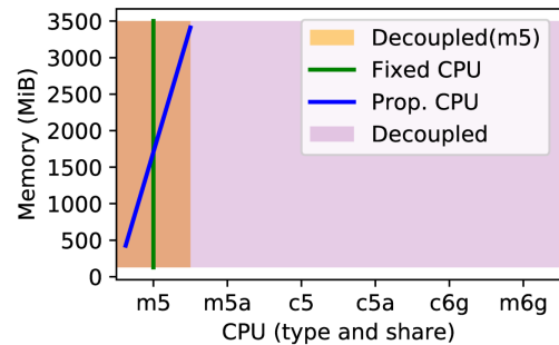
Figure 2. Four strategies for configuring serverless functions. Each strategy defines a search space, corresponding to a subset of the possible resource allocation configurations.
