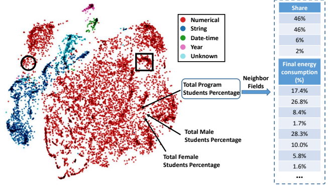
Figure 5: Visualization of Shared Table Representations.
