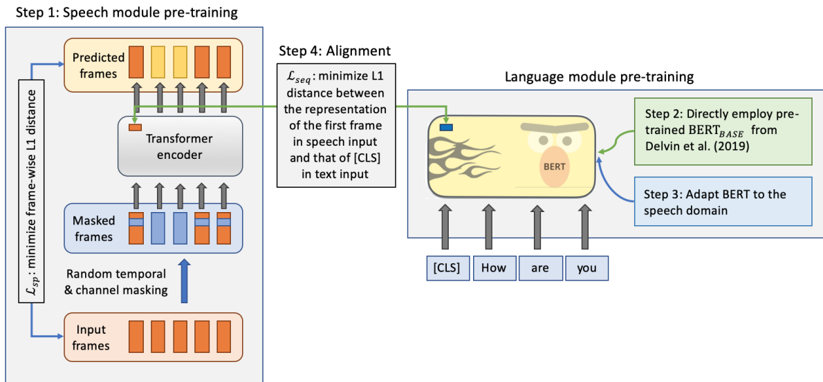
Figure 1: Overview of SPLAT. First, the speech and language modules are separately pre-trained using speech and text data via masked language modeling (MLM). In practice, we directly employ the BERT_{BASE} model released by Devlin et al. (2019) to be the language module. Then, by leveraging a small amount of paired speech and text data, either a sequence-level alignment loss \mathcal{L}_{seq} or a token-level alignment loss \mathcal{L}_{tok} is applied to align the representations from both modules in a shared latent space (only \mathcal{L}_{seq} is shown here). During alignment, the language module is kept frozen and only the speech module is updated. Before aligning the two modules, there is an optional step to update the BERT_{BASE} -initialized language module via MLM using the text portion from the paired data. This optional step aims to adapt the language module to the speech domain to facilitate later alignment. After pre-training, the language module is discarded and only the speech module is used in downstream tasks.
