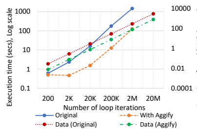
(b) MinCostSupplier (Java)
