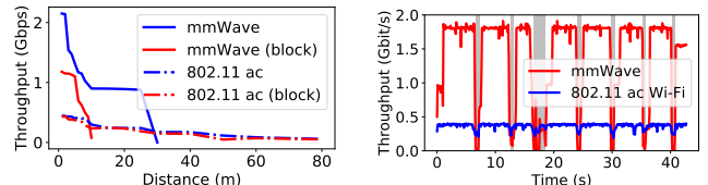
(a) TCP throughput at different link distances. (b) TCP throughput variation due to human blockage.
