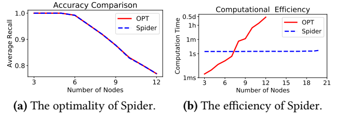
Figure 17: The optimality and efficiency of Spider flow planning algorithm.
