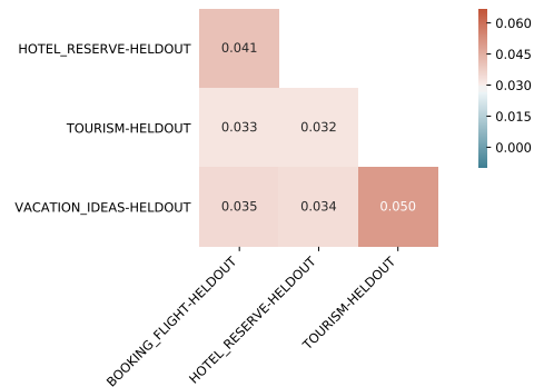
(b) Domain similarities for the MetaLWOz evaluation dataset.
