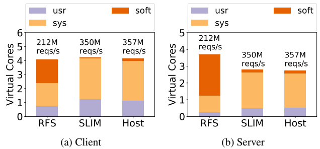
Figure 10: CPU utilization of Memcached client and server.
