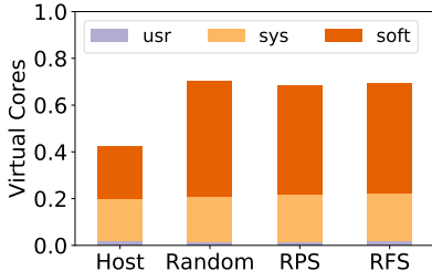
Figure 3: CPU utilization under different overlay network setups measured by number of virtual cores used for a single 10 Gbps TCP connection. The CPU cycles are spent: in user-level application (usr), inside kernel but excluding interrupt handling (sys), and serving software interrupts (soft).
