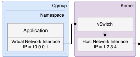
Figure 2: Architecture of container overlay network.
