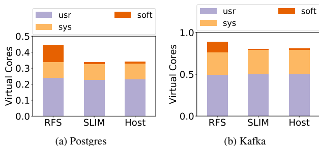
Figure 12: CPU utilization breakdown of the PostgreSQL server and Apache Kafka server.
