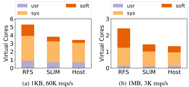
Figure 11: CPU utilization breakdown of the Nginx server.
