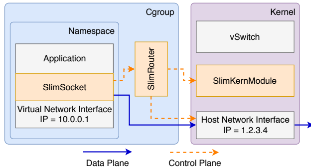
Figure 4: Architecture of Slim.
