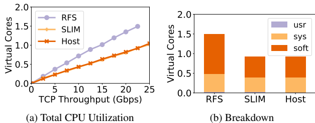
Figure 6: CPU utilization and breakdown for a TCP connection. In Figure 6a, the Slim and the host lines overlap. In Figure 6b, the usr bar is at the bottom and negligible.
