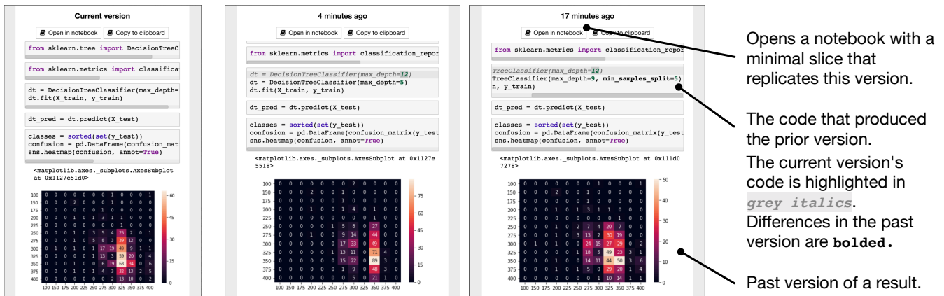
Figure 4: Comparing versions of a result with code gathering tools. When an analyst executes a cell multiple times, code gathering tools archive each version of the cell. When the analyst chooses the cell’s output—say, the confusion matrix shown above—and clicks “Gather to Revisions,” a version browser appears that lets them see all versions of that output, compare the code slices that produced each version, and load any of these slices into a new notebook, where the version’s results can be replicated.
