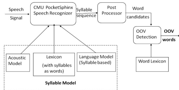
Figure 1: Syllable based decoding with post-processing for OOV detection.
