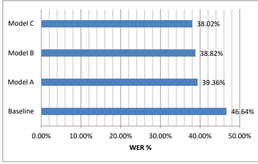
Figure 2: Wordmodel WER at using different stages of enhanced syllable-model ASR for OOV detection.
