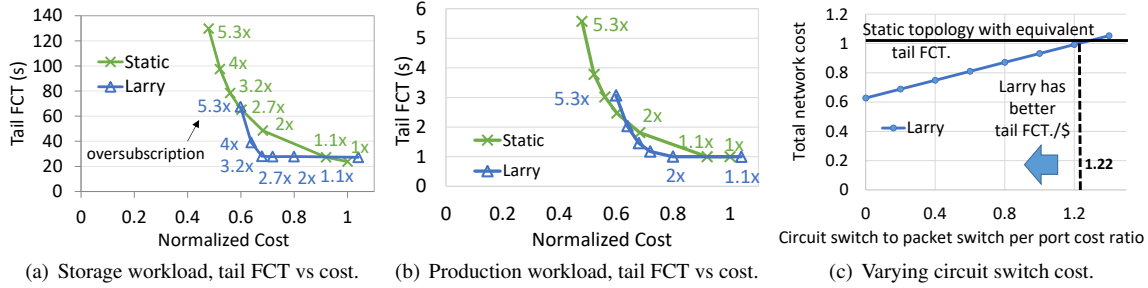
Figure 7: Performance as a function of cost.
