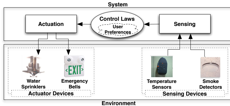
Fig. 11.3 Emergency control in buildings.
