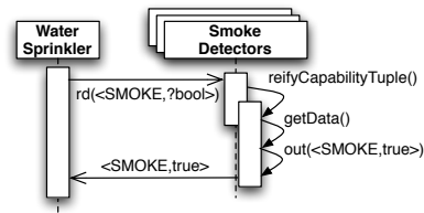
Fig. 11.5 Processing of capability tuples.
