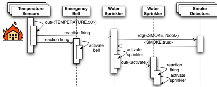
Fig. 11.4 Sequence of operations to handle a fire. Once notified about increased temperature, a node controlling water sprinklers queries the smoke detectors to verify the presence of fire. If necessary, it sends a command activating nearby sprinklers.
