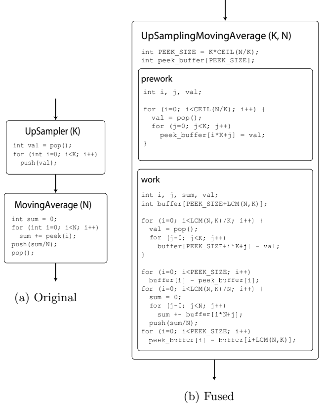
Figure 8: Vertical fusion with buffer localization and modulo-division optimizations.
