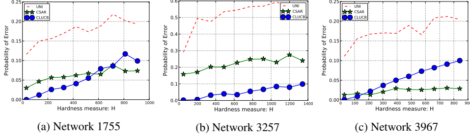
Figure 4: Comparison of empirical probability of errors with respect to \mathbf{H} .
