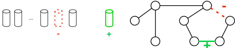
(a) An exchange set from \mathcal{B}_{\text{MATROID}(n)} (TOPK: Fact 2; each cylinder represents an arm).
